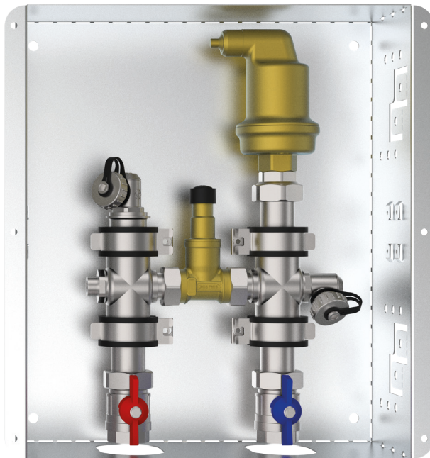
Loop ventilation with temperature maintenance
